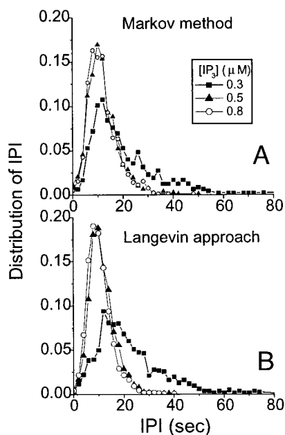
FIGURE 8 Interpuff-interval distributions of puffs obtained with the Markov method (A) and the Langevin approach (B) are shown at N = 20 and [IP_3] = 0.3 \mu M (solid square), 0.5 \mu M (solid triangle), and 0.8 \mu M (open circle).
