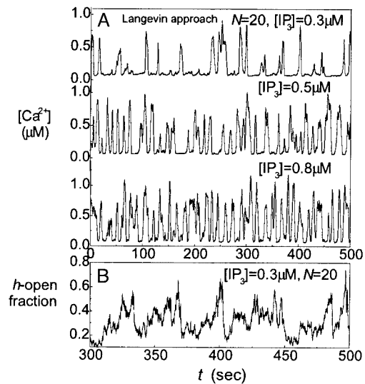
FIGURE 3 (A) Stochastic oscillation of the calcium release of a cluster of 20 \text{IP}_3 Rs with the Langevin approach is shown for [\text{IP}_3] = 0.3, 0.5 , and 0.8 \mu\text{M} . (B) The trace of the fraction of h -open channels for N = 20 and [\text{IP}_3] = 0.3 \mu\text{M} .
