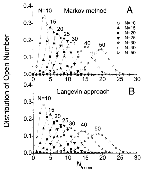
FIGURE 9 Distribution of h -open channel numbers for [IP_3] = 0.3 \mu M and various cluster sizes N = 10, 15, 20, 25, 30, 40 , and 50 with the Markov method (A) and the Langevin approach (B). For N = 20 , e.g., the most likely number of recruited channels of a puff is 7.
