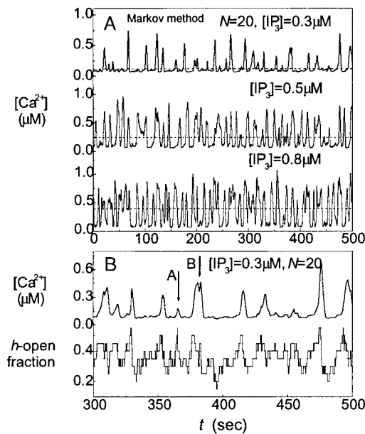
FIGURE 2 (A) Stochastic oscillation of the calcium release of a cluster of 20 \text{IP}_3 Rs obtained with the Markov method at [\text{IP}_3] = 0.3, 0.5 , and 0.8 \mu\text{M} . The dotted line is for the result obtained with the deterministic model. (B) A calcium trace is compared with the associated trace of the fraction of h -open channels for N = 20 and [\text{IP}_3] = 0.3 \mu\text{M} .
