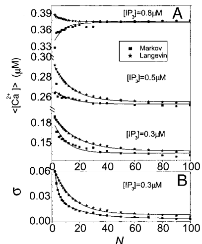
FIGURE 4 Time average of the calcium signal as a function of the cluster size N at [\text{IP}_3] = 0.30, 0.50 , and 0.8 \mu\text{M} (A). Variance of the calcium signal as a function of the cluster size N at [\text{IP}_3] = 0.30 \mu\text{M} (B). The results obtained with the Markov method and with the Langevin approach are marked by solid squares and stars, respectively.
